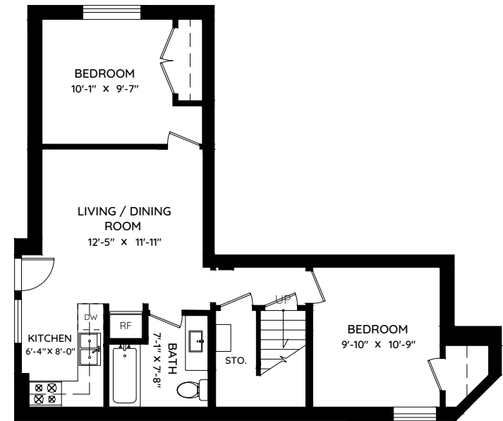
LOWER FLOOR 735 SQ.FT. CH: 8'-8"
